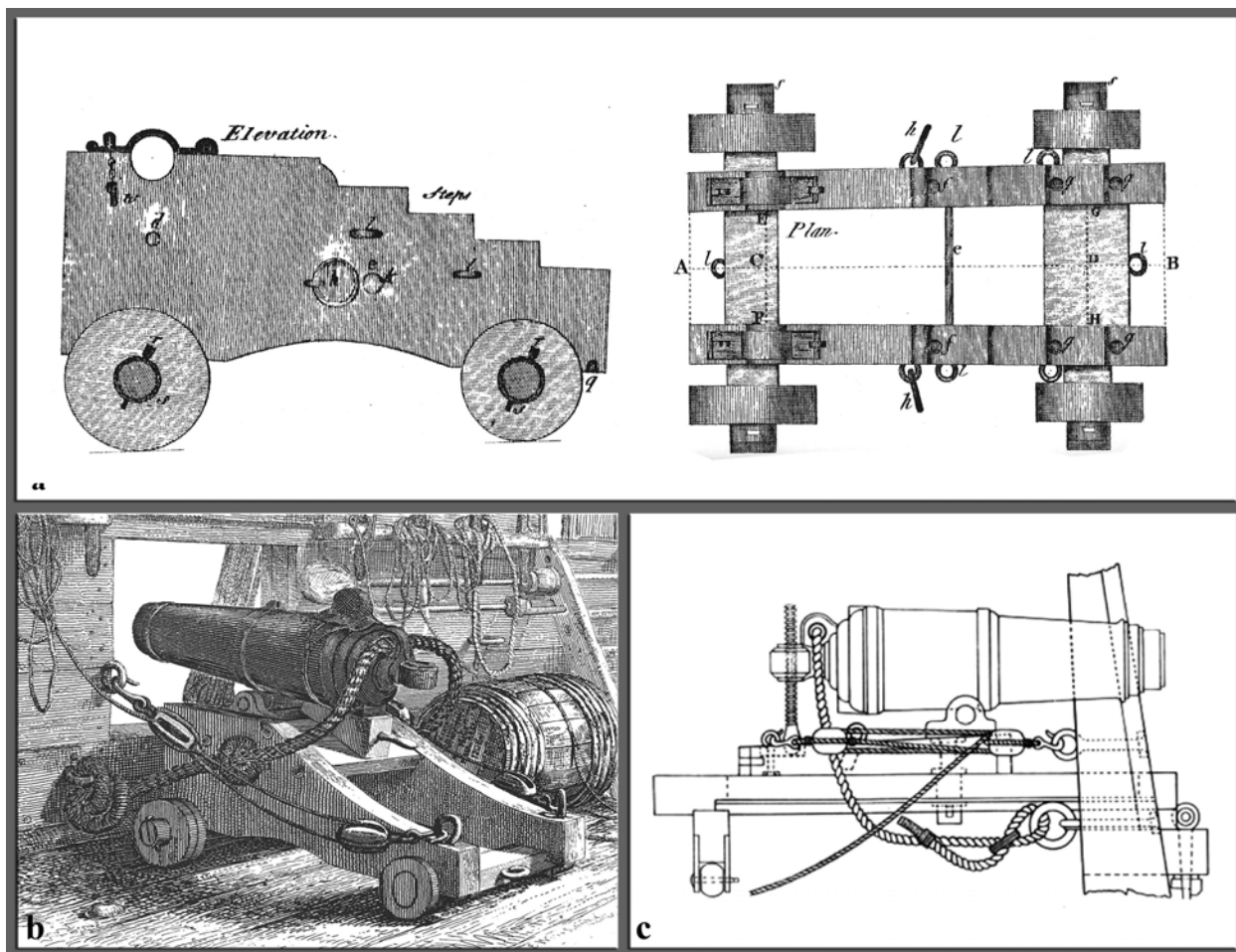
Figure 5.43. Naval Gun Carriages. (a) typical naval carriage (Muller 1995:94 [1780]) (b) early nineteenth-century 12-pound carronade (Cooke 1989:44) (c) bed and slide mount for a 24-pound carronade circa 1820 (Clowes 1900:540).
