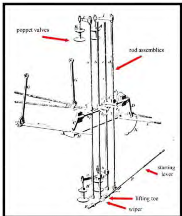
FIGURE 94. LIFTING ROD AND POPPET VALVE ASSEMBLIES. THE STEAM CHEST HAS BEEN OMITTED TO VIEW THE ASSEMBLIES; MODIFIED FROM INTERNATIONAL CORRESPONDENCE SCHOOLS (1897:69, FIG. 331)
