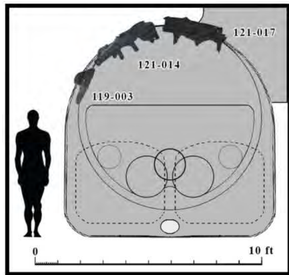
FIGURE 179. BOILER BARREL CONNECTION PLATES IN CONTEXT
