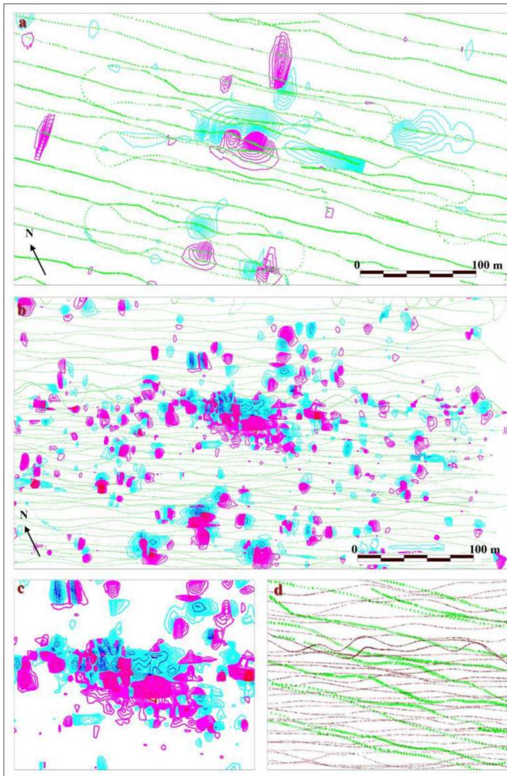
FIGURE 40. SURVEY OF USS WESTFIELD FROM (A) APRIL 2007 AND (B) JULY 2007; (C) DETAIL OF THE MAIN WRECK SITE; (D) COMPARISON OF SURVEY LINE RESOLUTION FROM APRIL 2007 (GREEN) AND JULY 2007 (BROWN).
