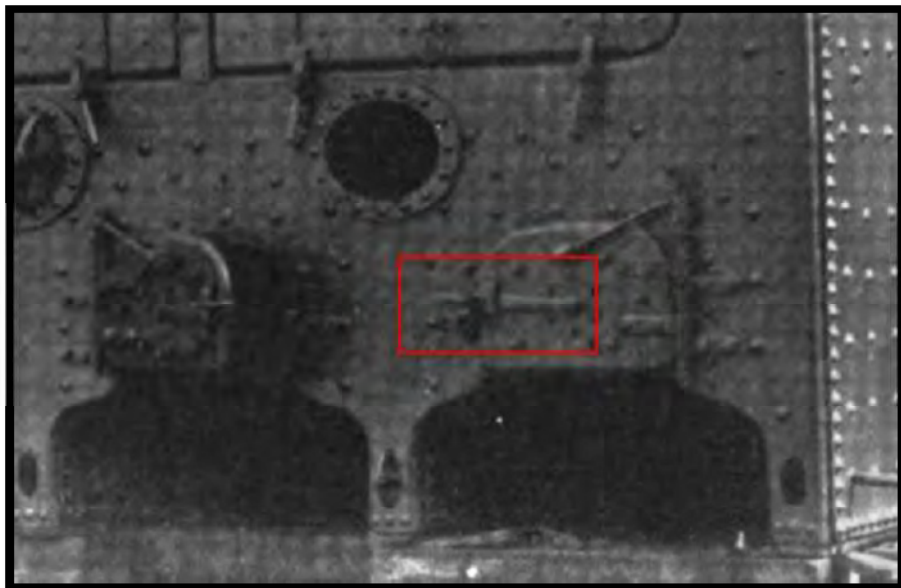
FIGURE 160. FIRE DOOR HAND LEVER ON PERRY BOILER (UNIDENTIFIED 1902:523)
