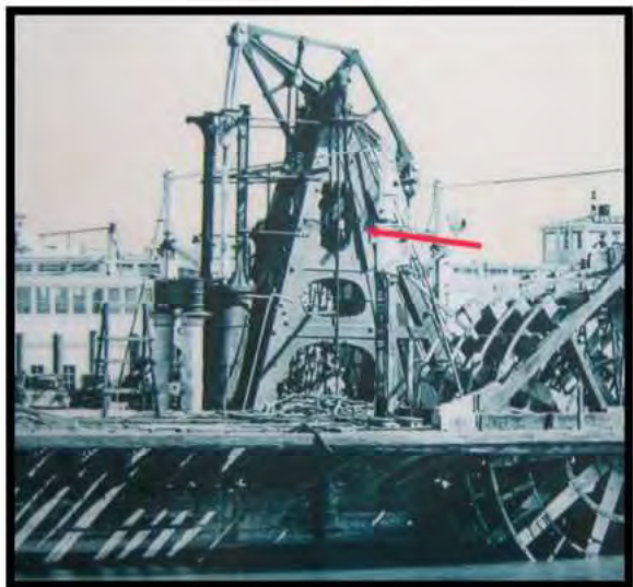
FIGURE 111. WALKING BEAM OF FERRYBOAT EUREKA - LARGE KNEES CREATED OVAL SHAPES IN THE A-FRAME (IMAGE COURTESY OF THE SAN FRANCISCO MARITIME NATIONAL HISTORICAL PARK)
